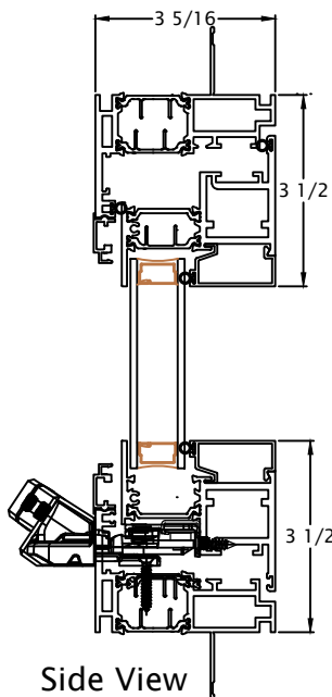
Block Frame Option
