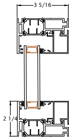
Block Frame Option Side View
