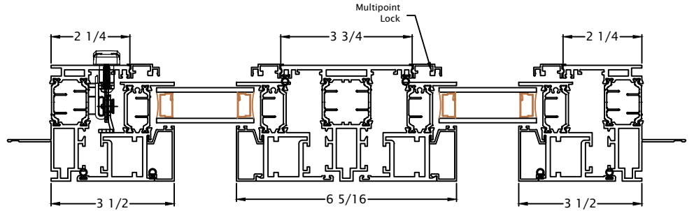
EXTERIOR CC Window Top View
