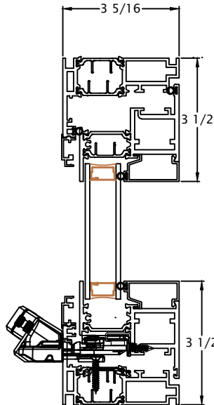
Block Frame Option
