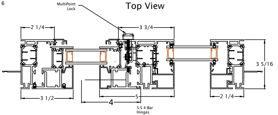
OC Window Top View
