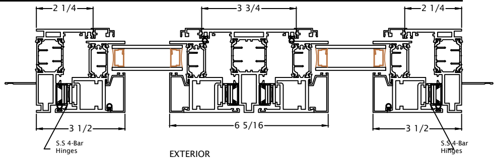
AA Window Top View
