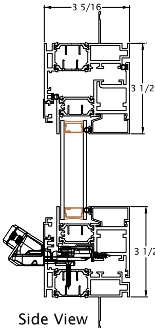
Block Frame Option
