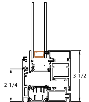
Block Frame Option 1" IG GLASS
