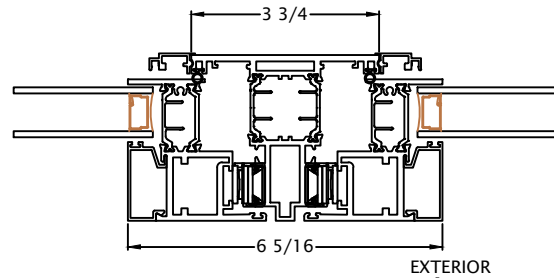
AA Window Top View
