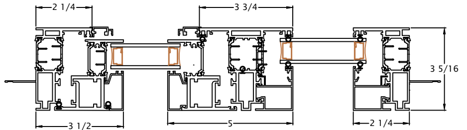
AA Window Top View
