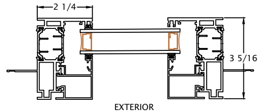
Top View Fix Window
