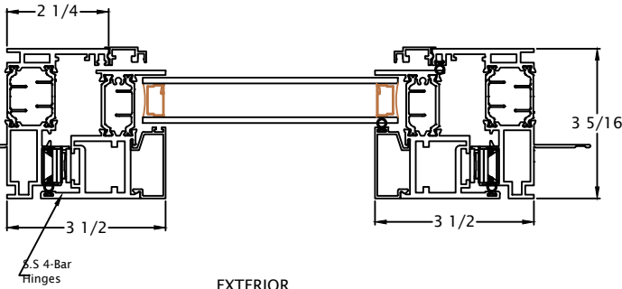
Awning Window Top View
