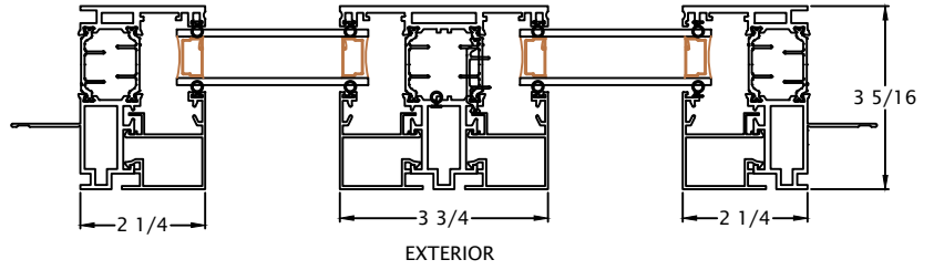
OO Window Top View
